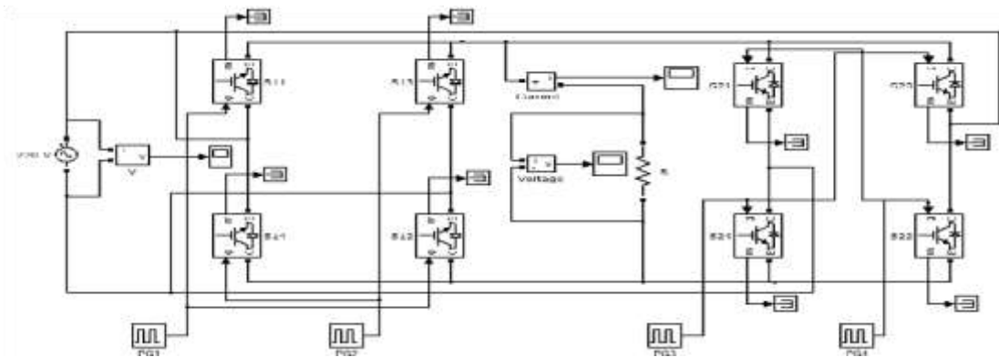
Fig.6: 1- phase to 1- phase cycloconverter
