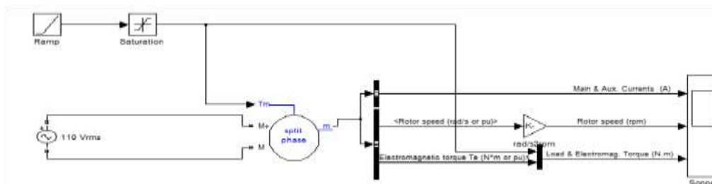
Fig.5: Split Phase Induction Motor
