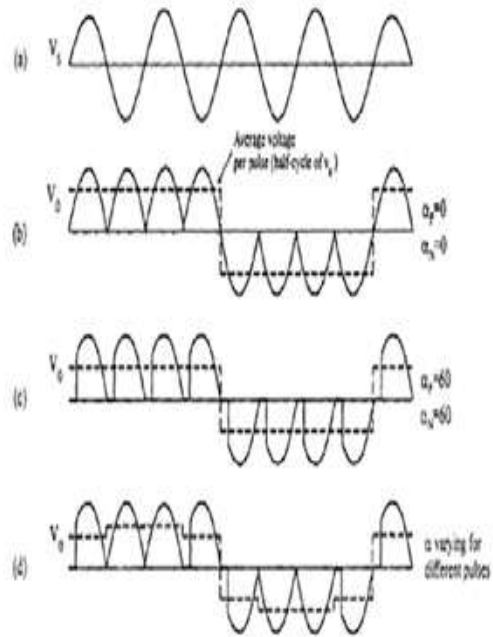
Fig. 2: Single Phase Cycloconverter Outputs a) Input voltage b) Output voltage for zero firing angle c) Output voltage for firing angle of 60 degrees d) Output voltage with varying firing angle
