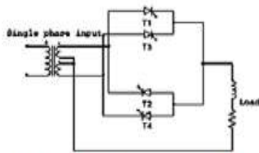
Fig.1: Single-phase input cycloconverter
