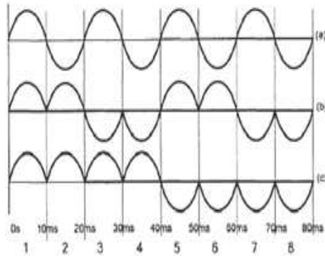
Fig.3: (a) Input 50Hz (b) Output 25Hz (c) Output 121/2Hz
